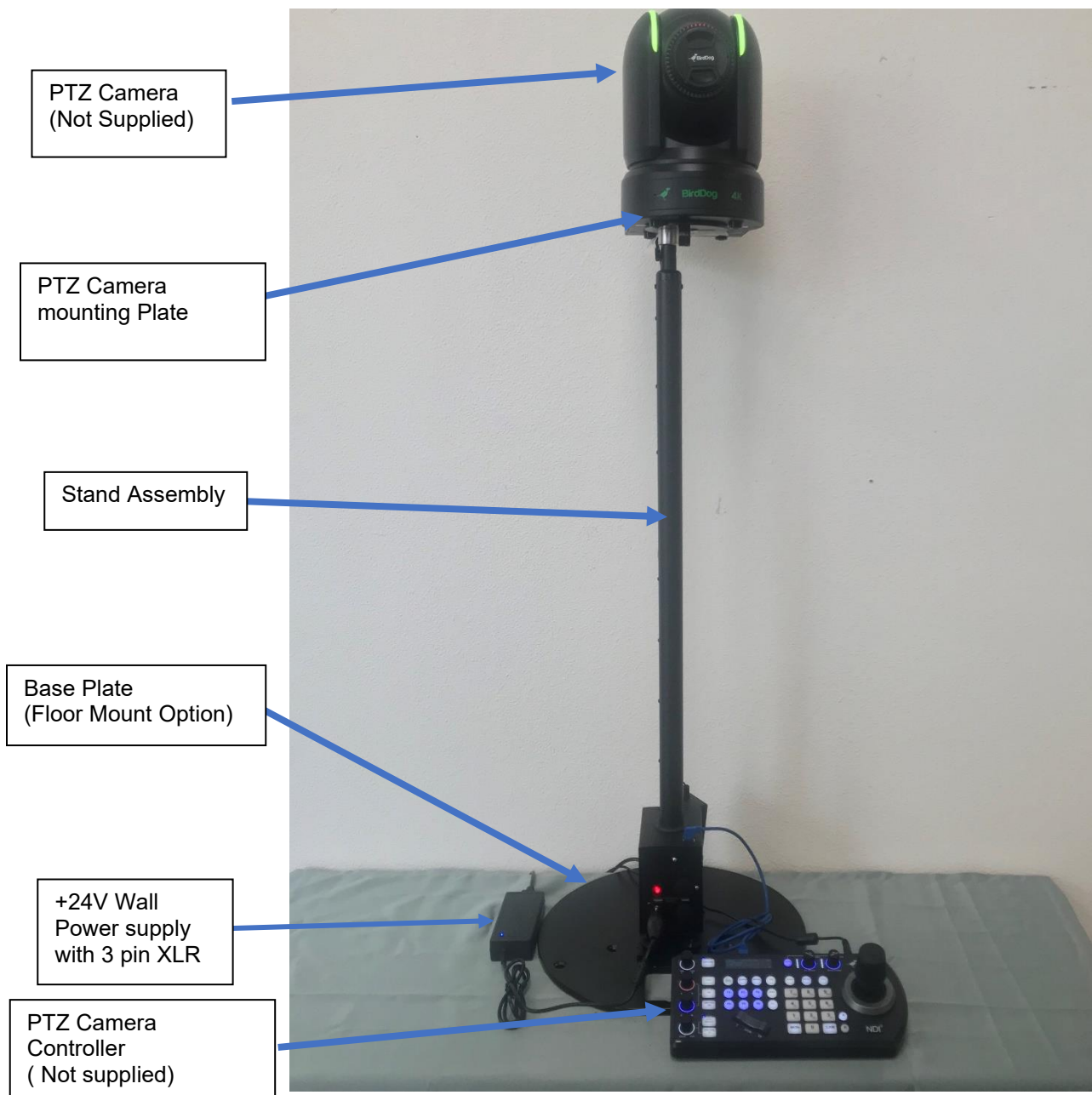
24" PTZMoverIP with Floor Mounted Baseplate
