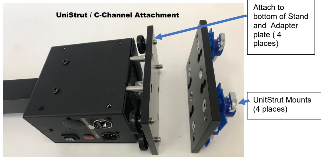
Ceiling Mounting, UniStrut or C channel
