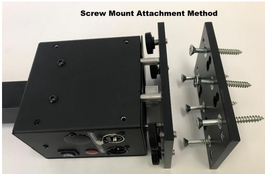
Ceiling Mounting, Screws
