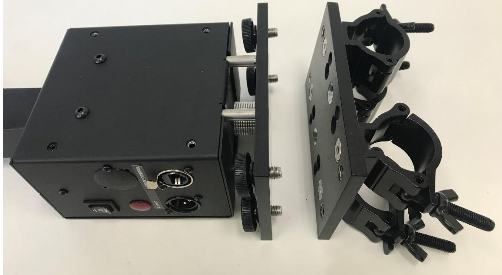
Ceiling Mounting, Pipe Grid
