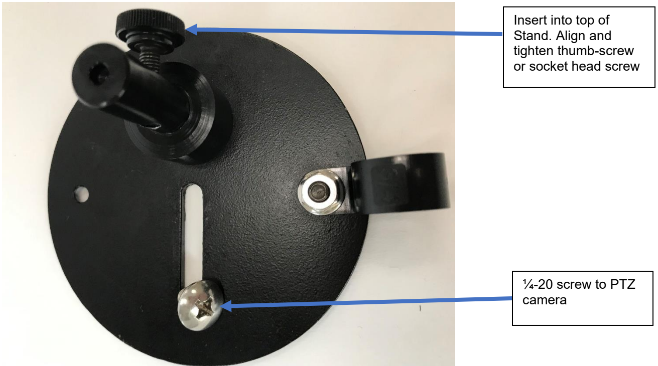
Figure 3 : PTZ Camera Adapter Plate ( bottom view)
