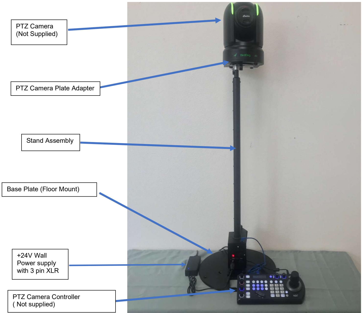
Figure 1: 24" PTZMoverIP with Floor Mounted Baseplate
